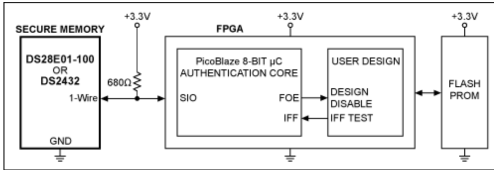
Figure 1. Simplified schematic of a Maxim 1-Wire memory device providing secure control and protection for an FPGA.
