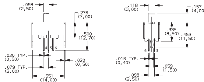
OS202011MV4QN1 DPDT
