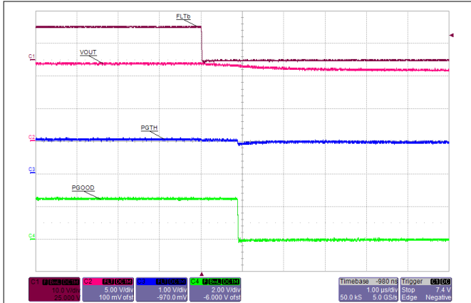
Figure 10-17. Power Good Response During Turn-Off
