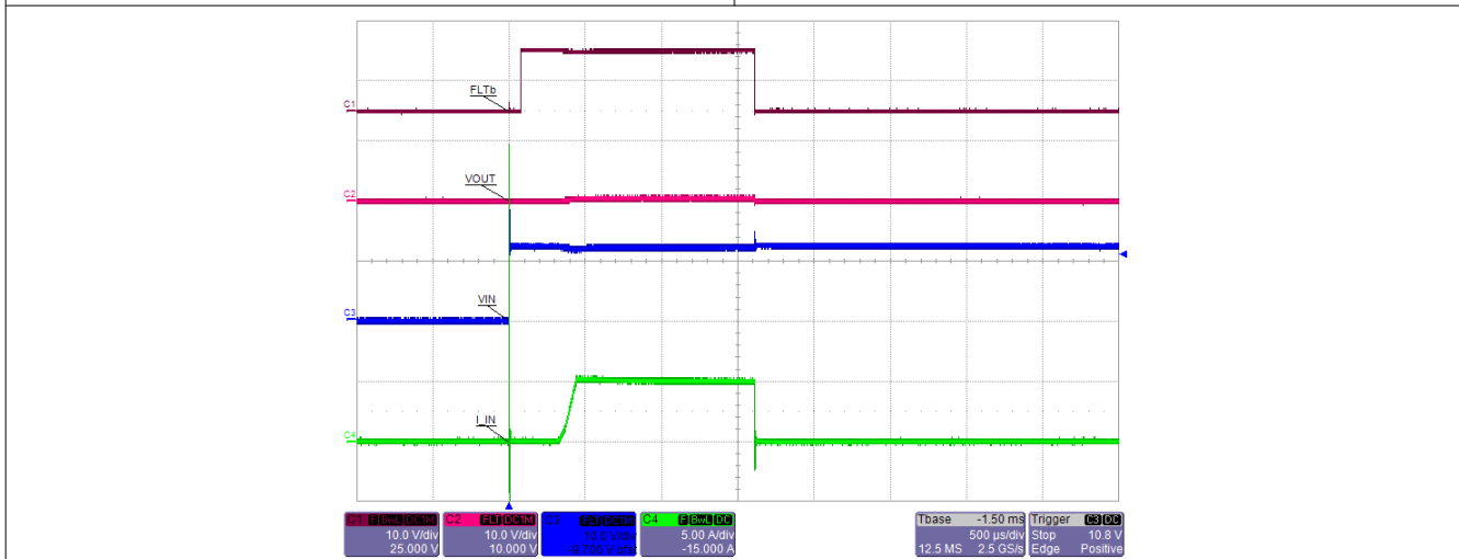
Figure 10-19. Hot Plug-in with Short on Output: Latched - TPS25940L-Q1
