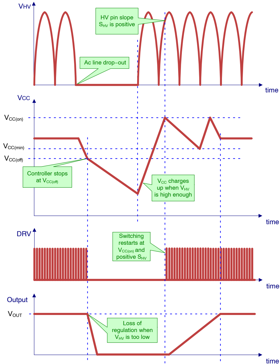
Figure 47. Ac Line Drop-out Timing Diagram
