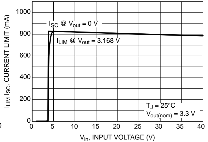
Figure 17. Output Current Limit vs. Input Voltage
