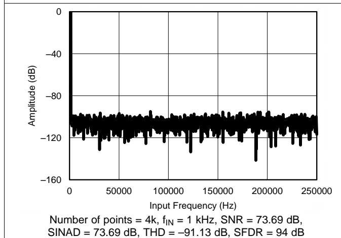
Figure 42. Typical FFT Plot ( \pm 2.5 \times V_{REF} )
