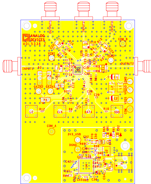
Figure 72. Silkscreen Top
